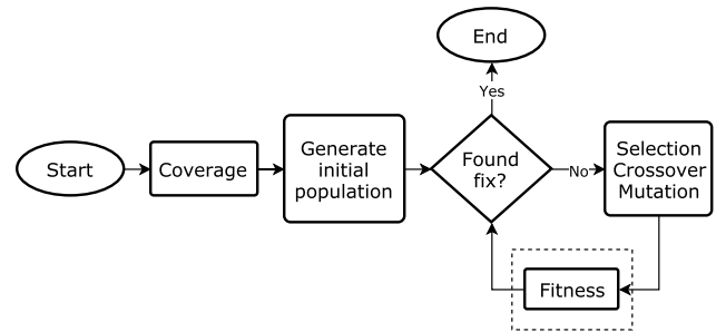
Figure 1: GenProg's algorithm.
