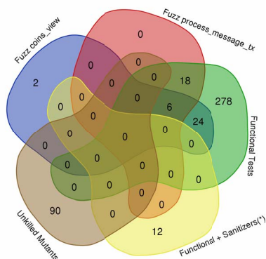
Figure 1: Mutation kills for tx_verify.cpp
